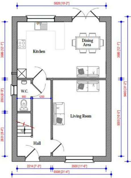
Ground Floor Plan 1:50
